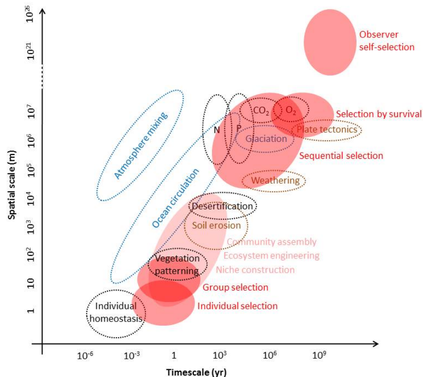
FIGURE 2. Space and timescales of Earth and Gaia processes. Some key Earth system processes are shown in blue (ocean-atmosphere) and brown (ocean-lithosphere). Examples of feedback mechanisms and regulated variables are shown in black. Selection and self-organisation mechanisms are shown in red.
